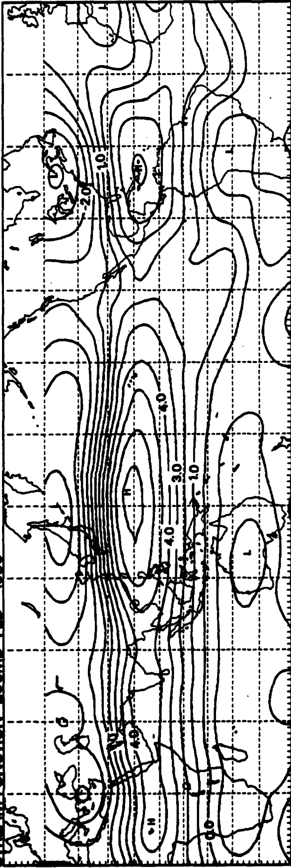
STREAM FUNCTION 200MB FEB 1980
